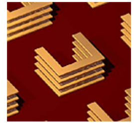
Concept drawing of stacked split-ring resonators made from gold and stacked on a glass substrate with polymer spacer layers.
